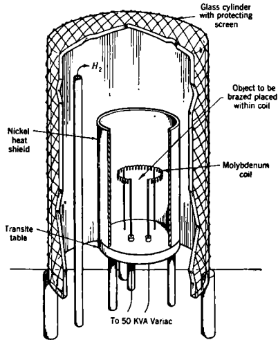
FIG. 17-12.—Hydrogen-bottle arrangement.
